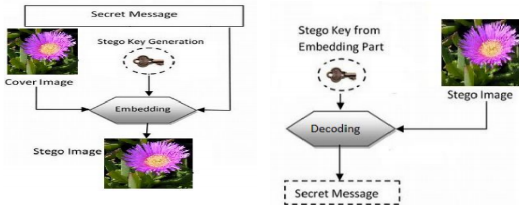
Fig.2. Block diagram of Image steganography[4]
