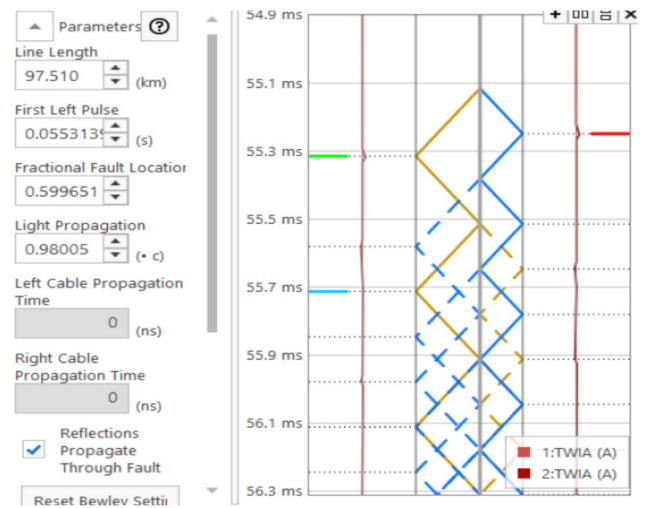
Fig. 14. Travelling wave characteristics at 60% location with T400
