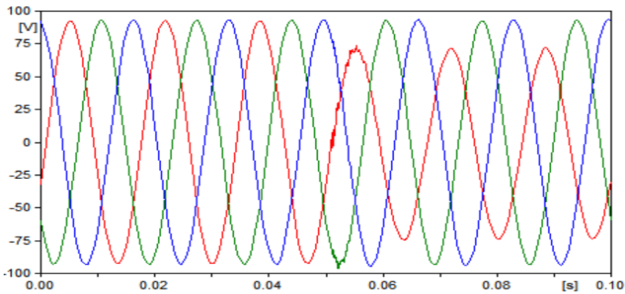
Fig. 7. Measurement voltage from Shinjecheon at 60% location of line
