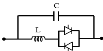
Fig. 1. Typical TCSC system
