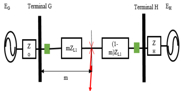
Fig. 2. One-line Diagram of a Two-terminal Transmission Network
