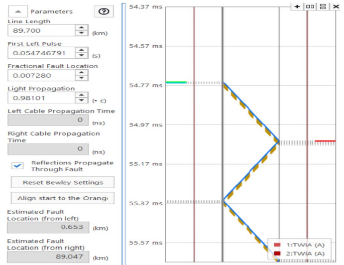
Fig. 16. Travelling wave characteristics at 0% location with T400
