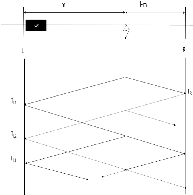
Fig. 11. Travelling wave characteristics at both ends
