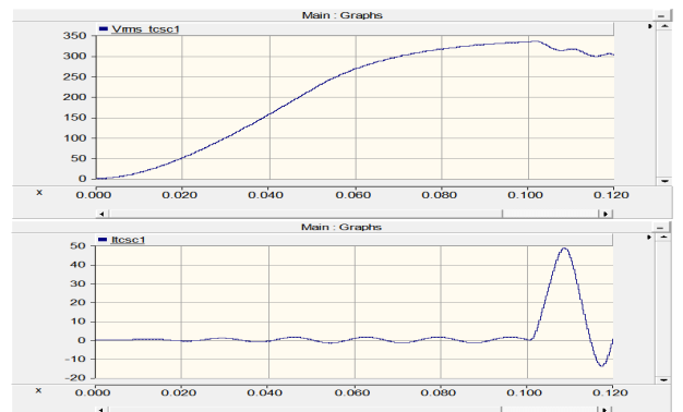
Fig. 5. Vrms and I waveform at 0% Shinjecheon-Donghae line location
