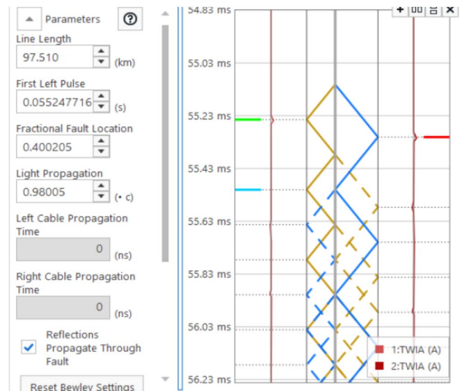
Fig. 13. Travelling wave characteristics at 40% location with T400
