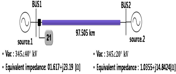
Fig. 6. Equivalent AC line for simulation of Shinjecheon-Donghae line
