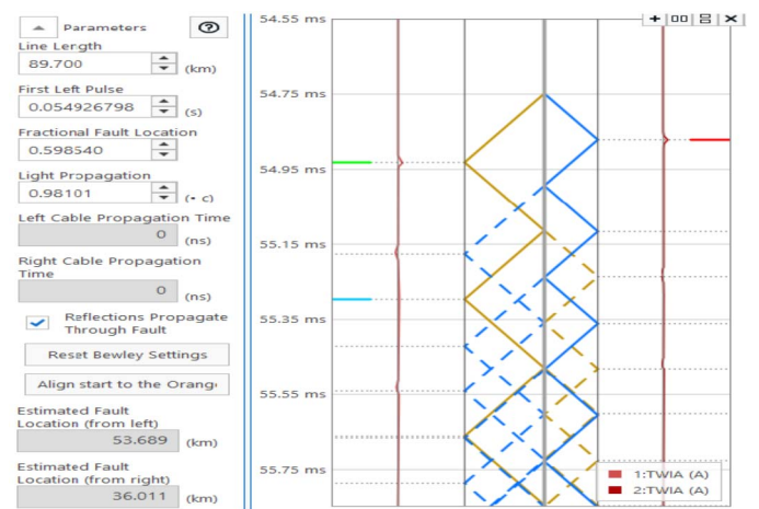
Fig. 18. Travelling wave characteristics at 60% location with T400
