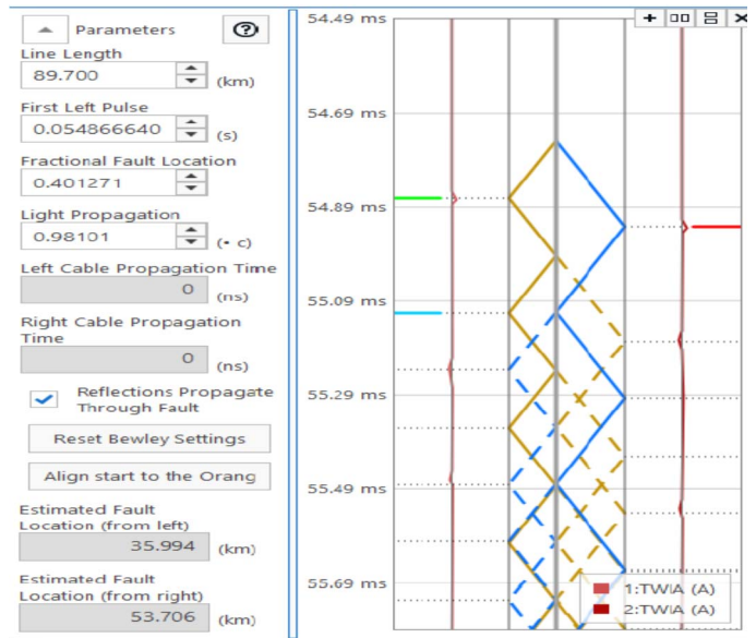
Fig. 17. Travelling wave characteristics at 40% location with T400
