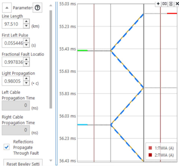
Fig. 15. Travelling wave characteristics at 100% location with T400
