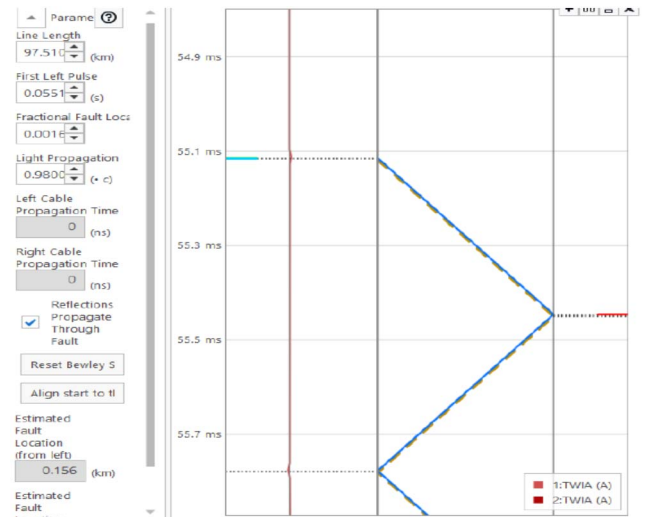
Fig. 12. Travelling wave characteristics at 0% location with T400
