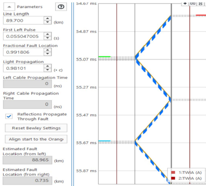
Fig. 19. Travelling wave characteristics at 100% location with T400
