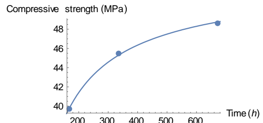
Figure 30. Compressive strength obtained at 28 days for SC + 10% wc; a / c = 0.45 and adjustment curve with exponential function.
