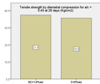
Figure 33. Results of tensile strength at 28 days for a / c = 0.45
