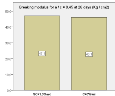
Figure 36. Results of tensile strength at 28 v days for a / c = 0.45
