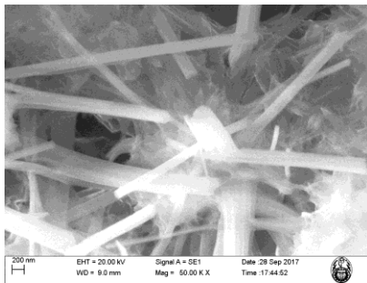
Fig. 9. Observation in scanning electron microscope SEM of sample SC + 1.0% wc at age 7 days for a / c = 0.45, with an amplification of 50 000x
