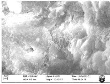
Fig. 14. SEM scanning electron microscope observation of sample C + 0.0% wc at age 28 days for a / c = 0.45, with an amplification of 10,000
