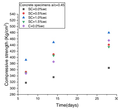
Figure 29. Compressive strength values obtained at 7, 14 and 28 days for a / c = 0.45
