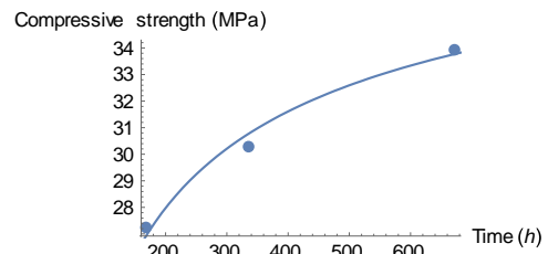
Fig. 25. Compressive strength obtained at 28 days for SC + 10% wc; a/c = 0.60 and adjustment curve with exponential function.
