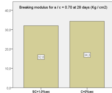
Figure 34. Breaking modulus results at 28 days for a / c = 0.70
