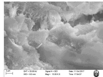
Fig. 12. Observation in scanning electron microscope SEM of sample SC + 1.0% wc at age 28 days for a / c = 0.45, with an amplification of 10 000x
