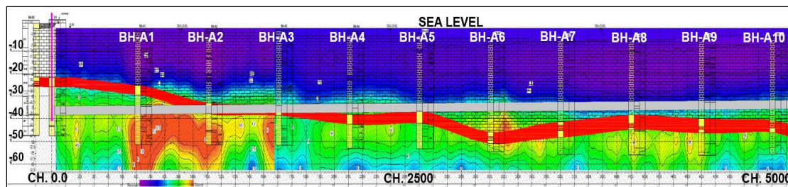
Figure 8: ERT line from 0 to 10.2 km
