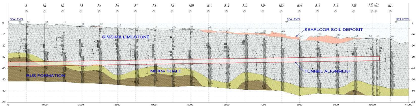
Figure 2: Lithological Cross Correlation from drilled bore holes
