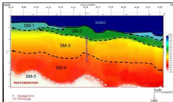
Figure 4: Seismic velocity section
