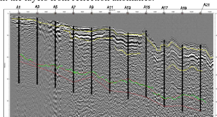
Figure 6: Seismic reflection cross section and bore holes
