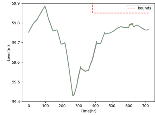
Figure 12. Robustness analysis on level control at Dalsfoss power station using the reference region tracking MPC with output constraints
